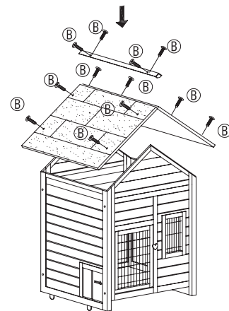
Step 3. Secure roof and ridge cap
